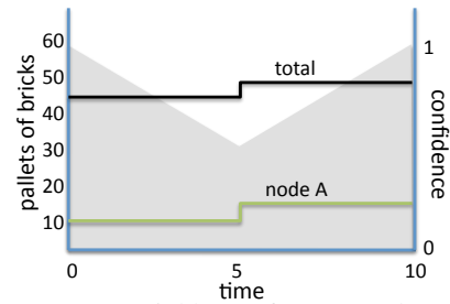
Fig. 8: Nearest Neighbor Inference and Confidence
