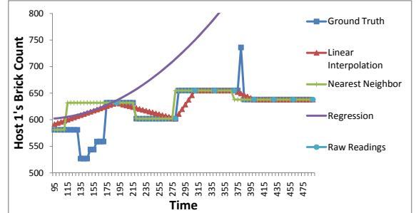
Fig. 11: Number of Bricks Sampled and Inferred for One Host
