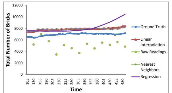
Fig. 12: Inferring an Aggregate over Time
