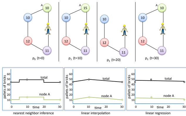
Fig. 6: Comparison of Types of Inference
