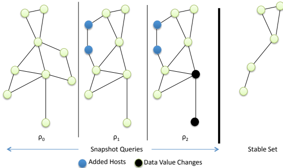
Fig. 1: A Continuous Query
