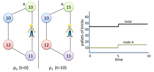
Fig. 4: Nearest Neighbor Inference for Uncertain Data
