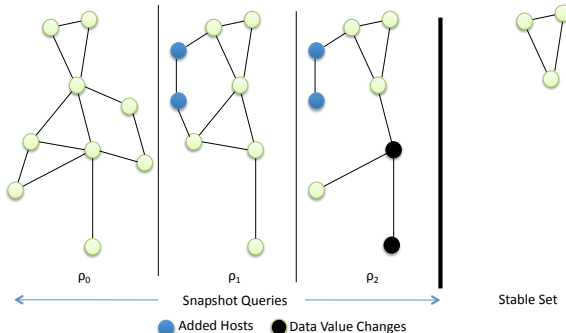
Fig. 2: A Continuous Query with Missing Data
