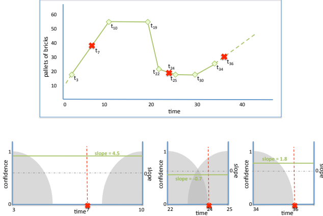
Fig. 9: Associating Confidence with Inferred Values
