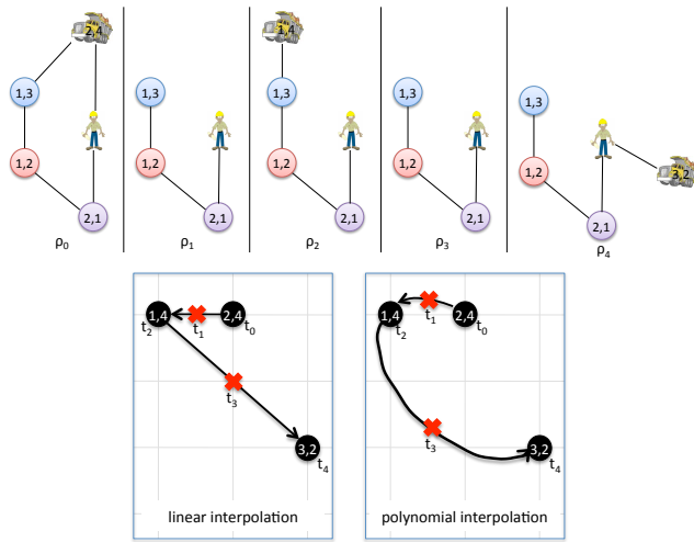
Fig. 5: Interpolation of Missing Location Data
