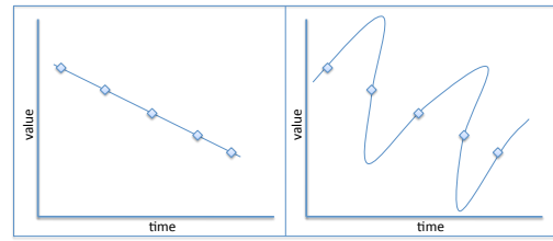
Fig. 7: Interpolation Error
