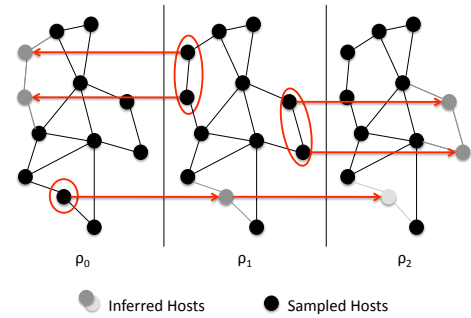
Fig. 3: Projection Forward and Backwards in Time
