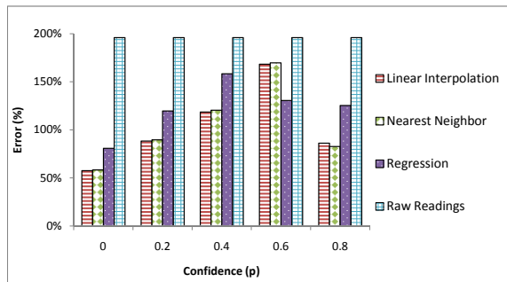
Fig. 13: Inferencing Error vs. Confidence
