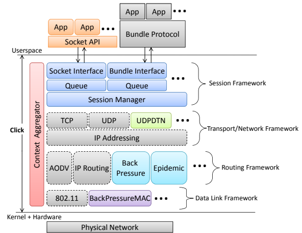
Figure 1: The MaDMAN Architecture
